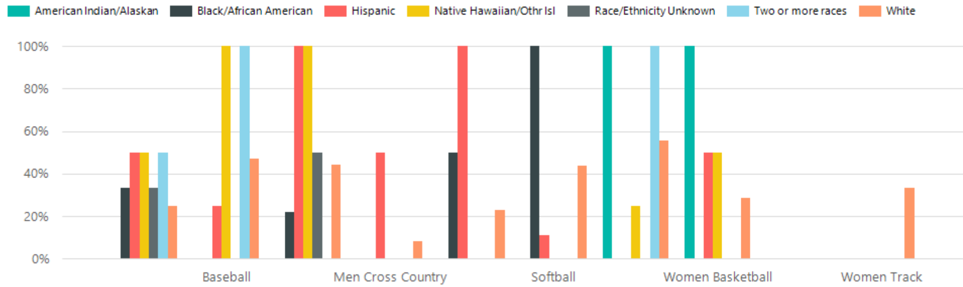
Transfer Rate
