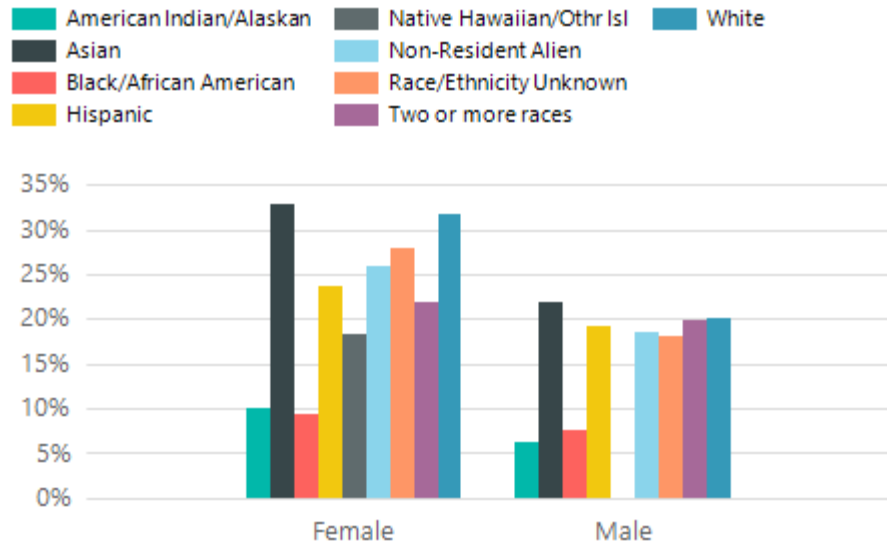
GraduationRate
