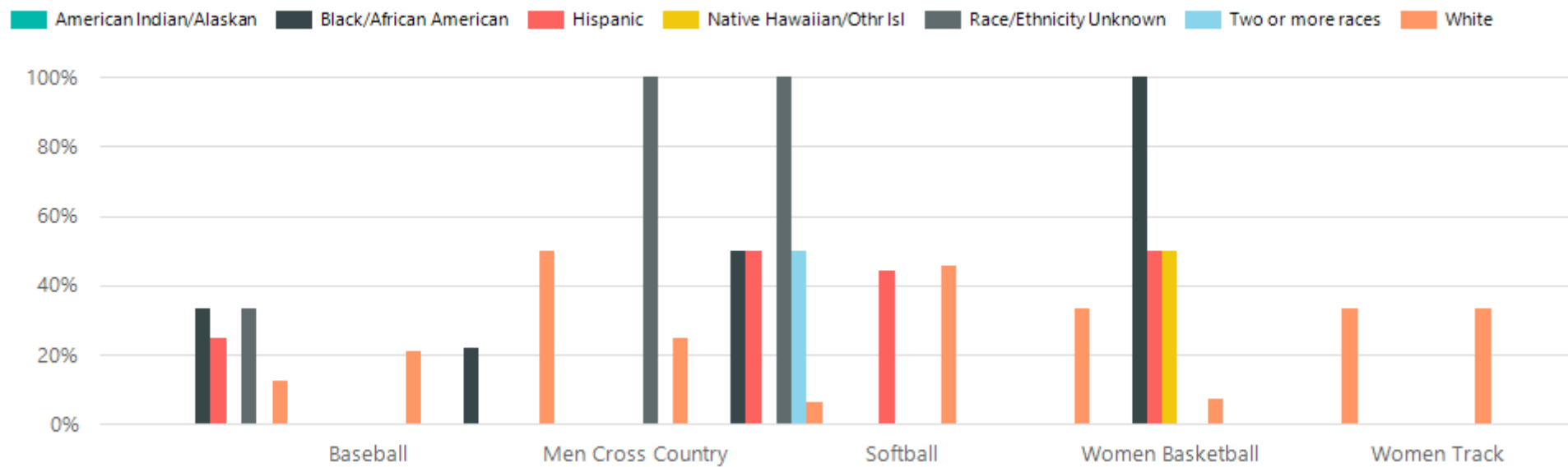
Graduation Rate
