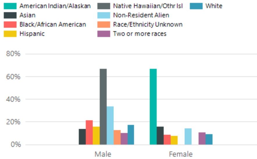
Transfer Rate
