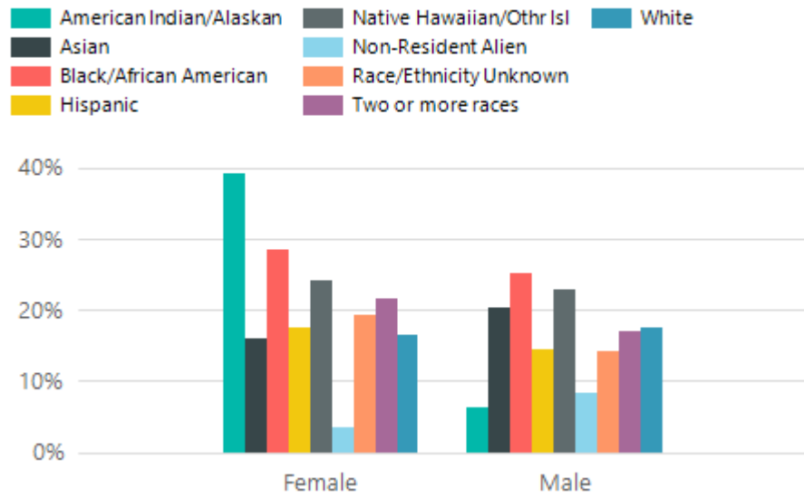
Transfer Rate
