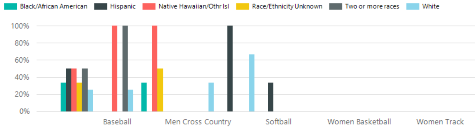
Transfer Rate
